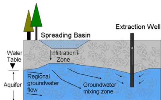
Artificial recharge through a spreading basin in an unconfined aquifer. Stored water is recovered through a well or allowed to discharge into a stream at some point downgradient. (Image courtesy of Oregon Water Resources Department).
