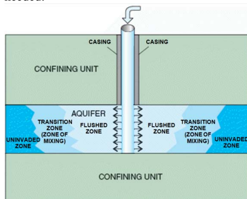
Aquifer storage and recovery well in a confined aquifer. Flushed zone contains mostly recharged water. (Image courtesy of USGS)
